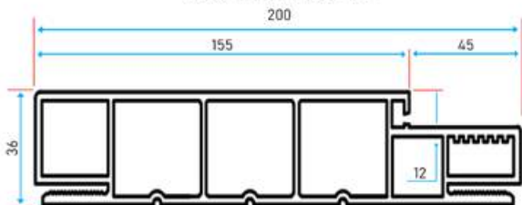
200 mm Frame
