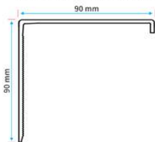
90*90 mm Architrave
