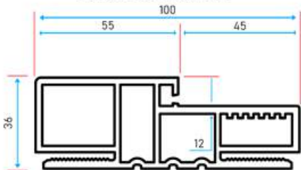
100 mm Frame
