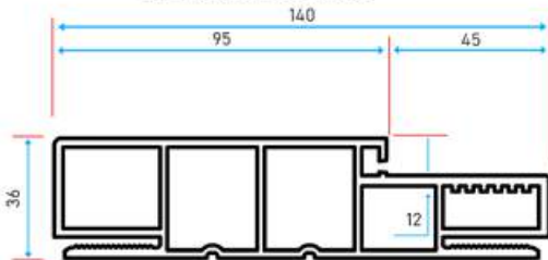
140 mm Frame
